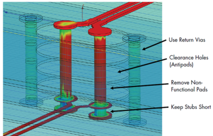
Optimal Differential Via Layout Example
