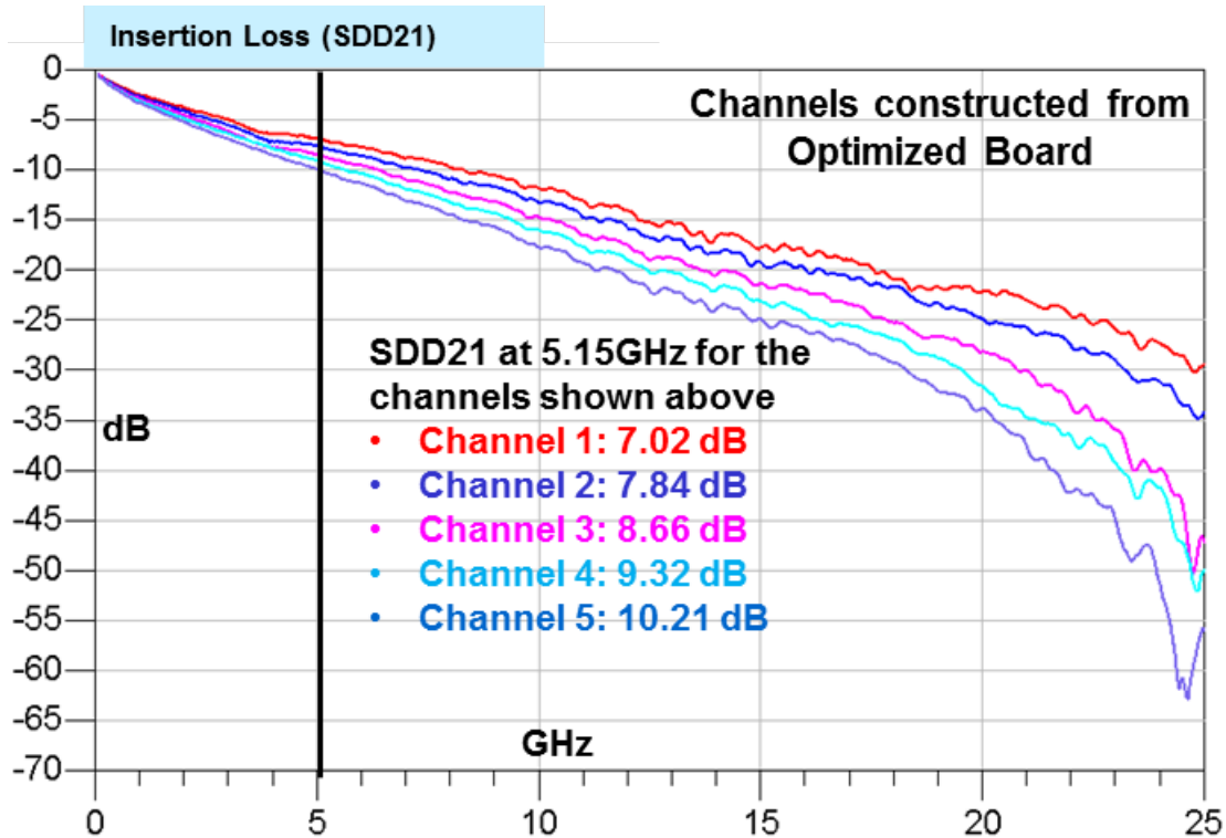
Figure 16: Impact of Insertion Loss on ISI
